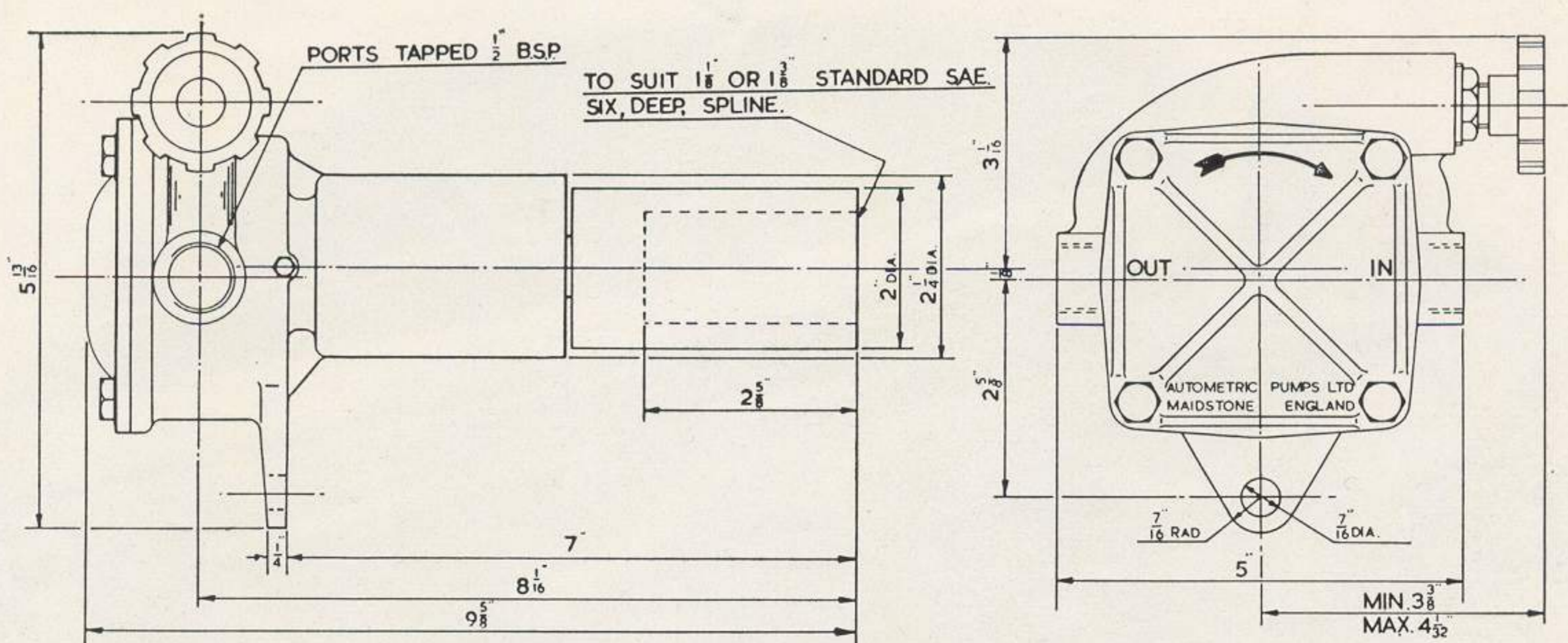
DIMENSIONS OF THE RS50/HV UNIT.
