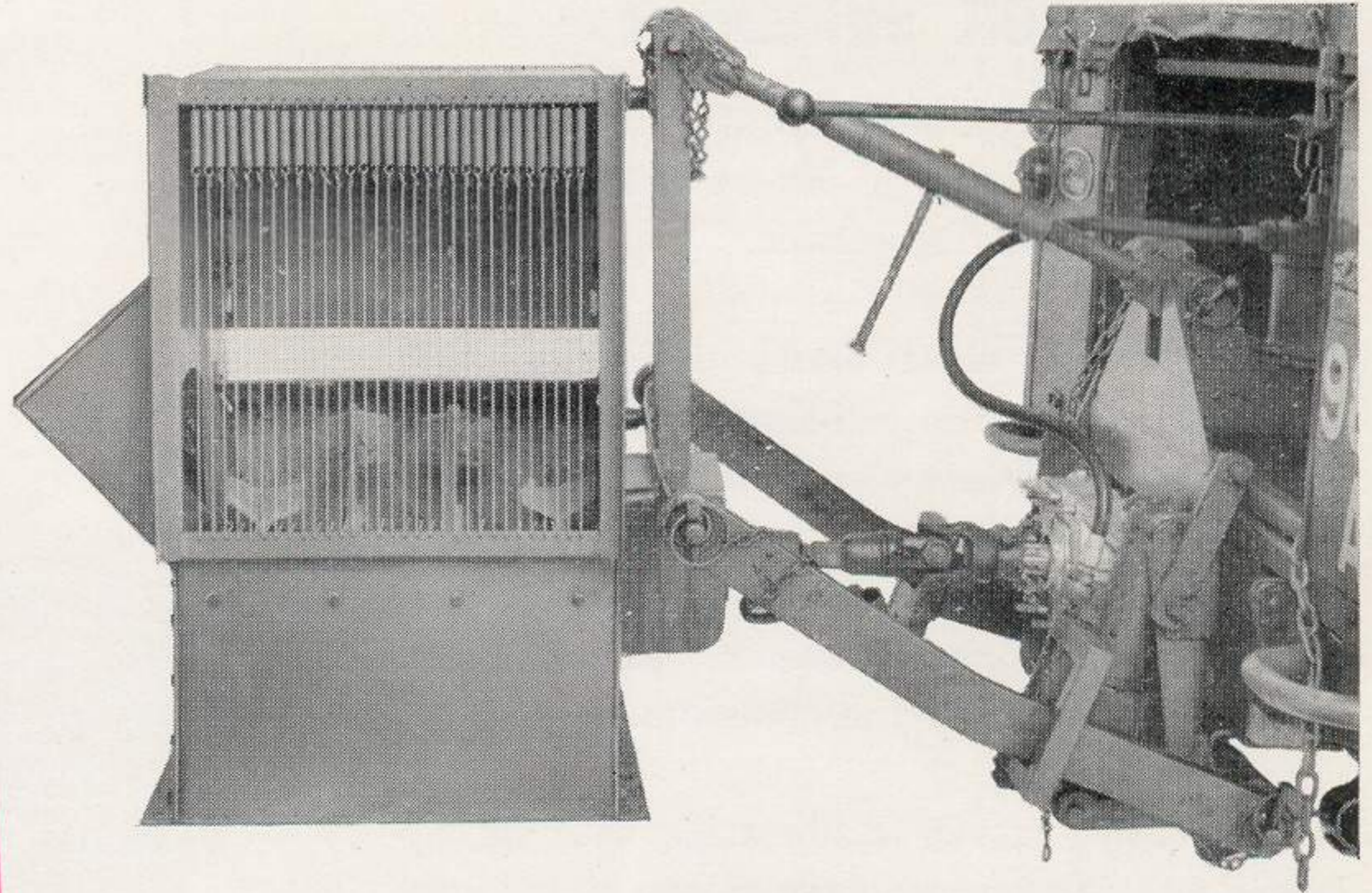
Mark 3R Shredder mounted on Land Rover 3-point linkage and with drive from rear p.t-o shaft.
