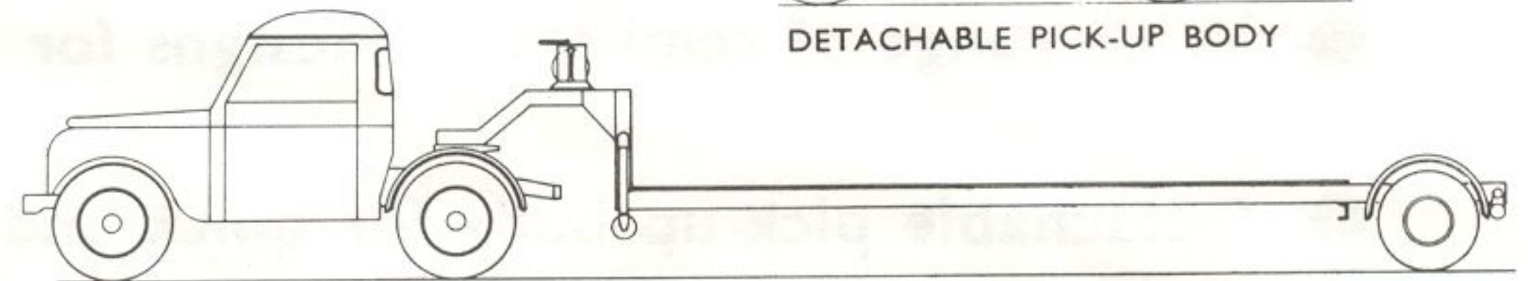
LOW LOADING WITH DETACHABLE AXLE FOR LIGHTWEIGHT BULKY LOADS
