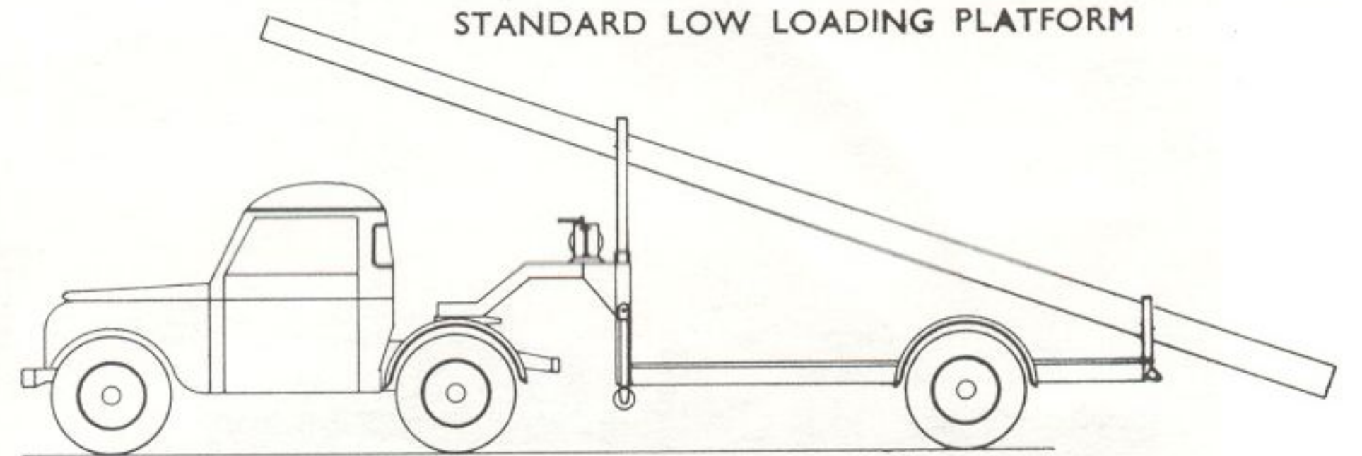
STANDARD LOW LOADING WITH POLE SUPPORTS
