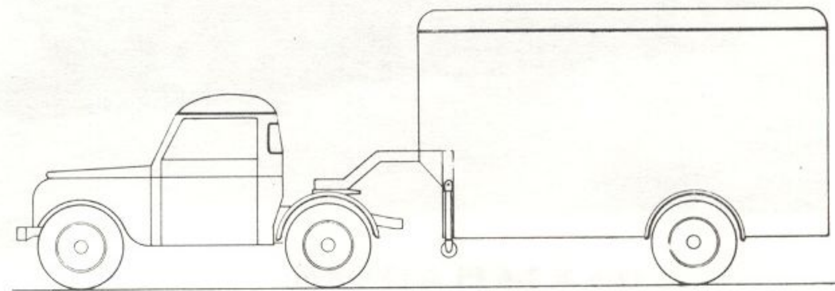
STANDARD LOW LOADING VAN
